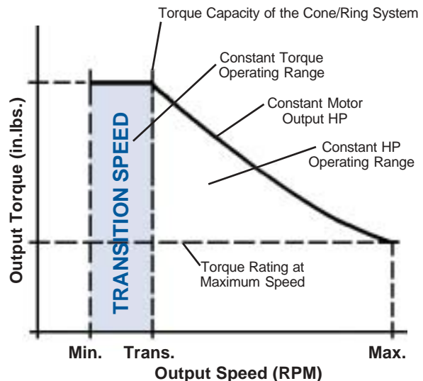
Graph No. 1 ComTrac Performance Chart
