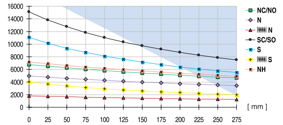
Gripping force as a function of jaw length [N]
