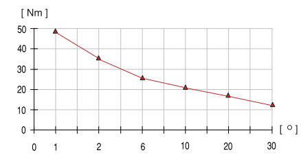
Gripping force as a function of opening angle
