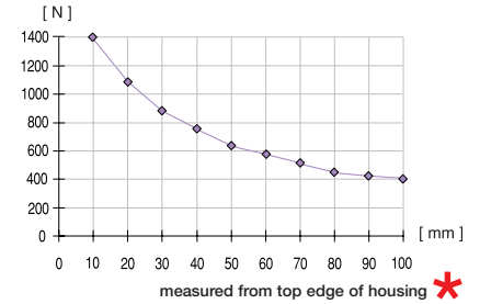
Gripping force as a function of jaw length (measured at 1° opening angle)
